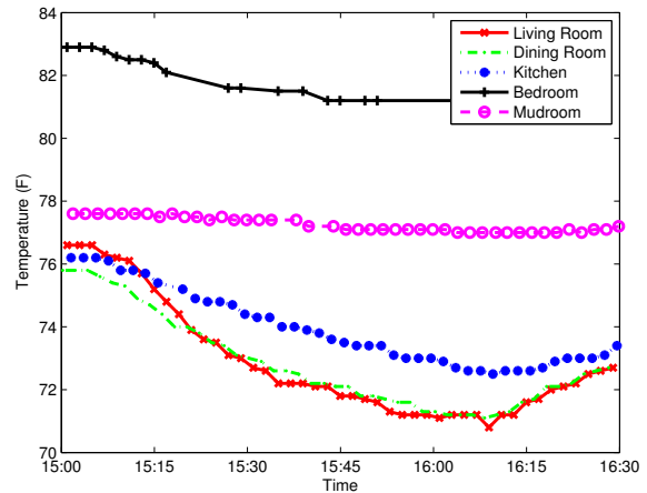
Figure 10. Temperature response of both conditioned and unconditioned rooms as the active zone temperature is dropped from 76 to 72.
